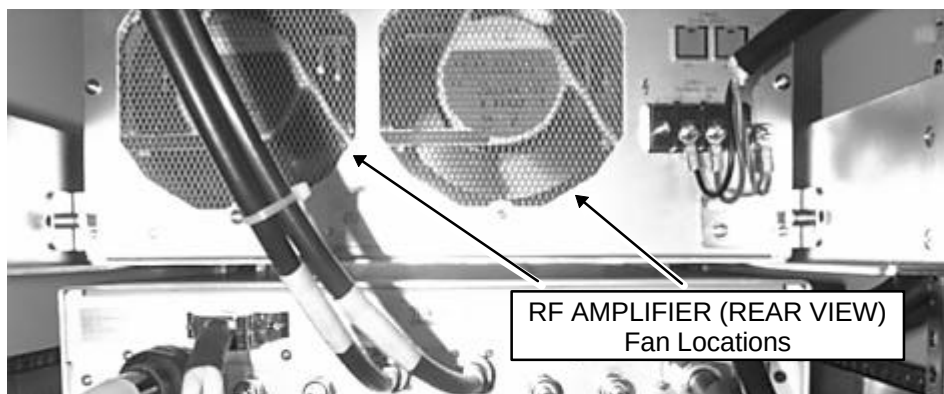
1.0T RF AMPLIFIER FAN LOCATIONS ILLUSTRATION 2-2
