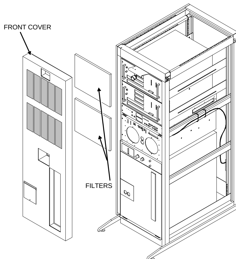
RF/PDU CABINET COVERS AND FILTER LOCATIONS ILLUSTRATION 2-1
